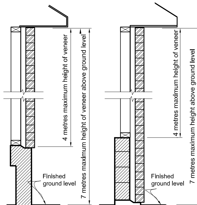
(b) 2 STOREY ON MASONRY
