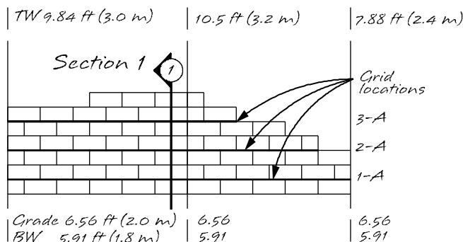
Wall Elevation - to identify grid locations
