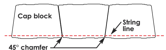
Install cap with an overhang to achieve a nice shadow line
