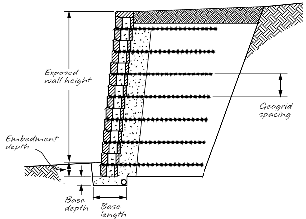
Typical Reinforcement Cross Section
