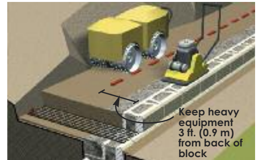
Keep heavy equipment away from the back of the block.
