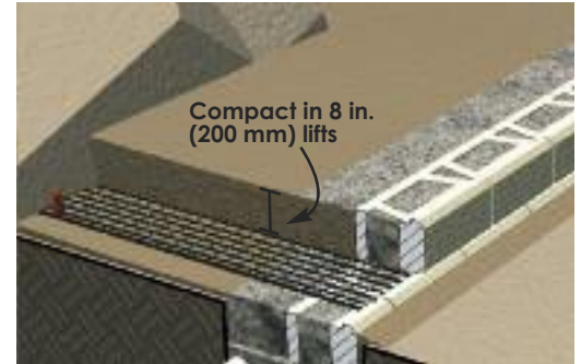
Compact in 8 in. (200 mm) lifts.
