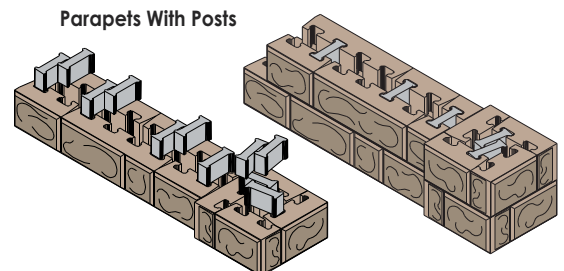
Posts within Parapets
