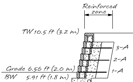
Wall Cross Section
