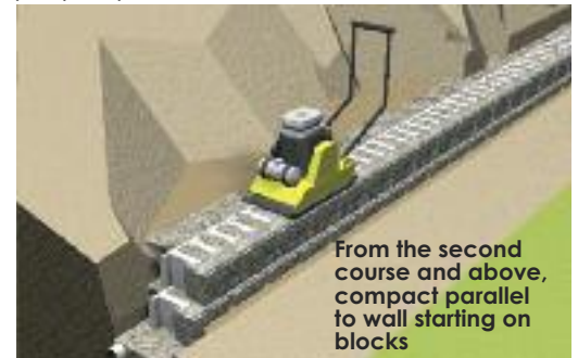
From the second course and above, compact parallel to wall starting on blocks. Compact wall rock and backfill soils starting on the blocks.
