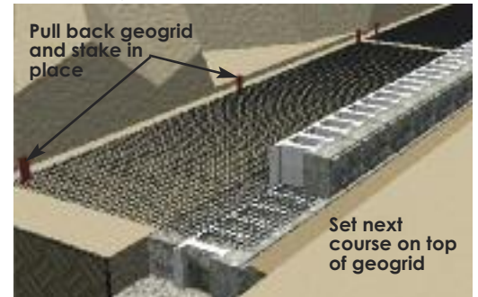
Stake geogrid in place. Install next course of block.
