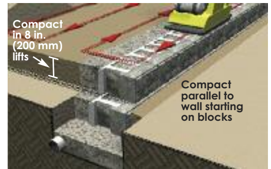
From the second course and up, compact starting on the wall and working to the back of the reinforced zone.
